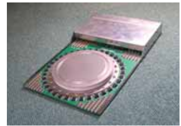
Gate Commutated Thyristor (GCT) with driver board. Rated 6,000 Volts, 6,000 Amps - the world's largest switching device
