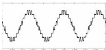
Line-to-Line Voltage at 100% Speed
