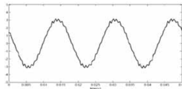
U-phase Current at 100% Speed
