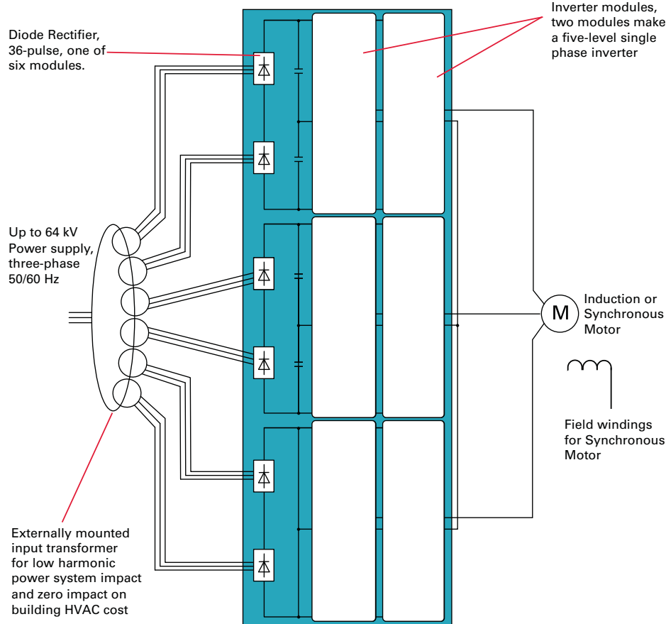
XL Architecture using Diode Converter and five-level Pulse Width Modulated Inverter
